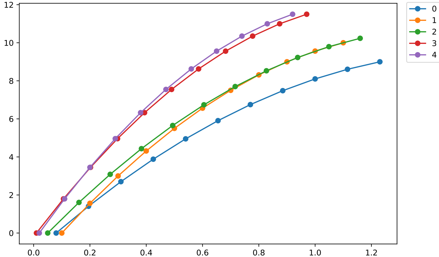
nonlinear0's curves with offsets at index 0
